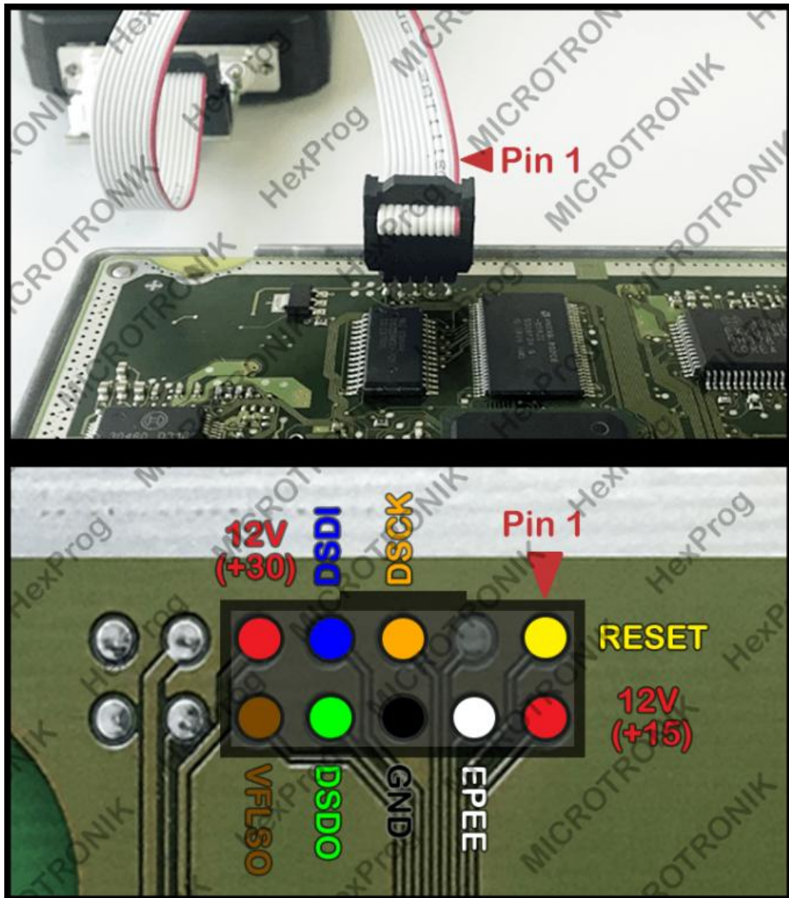
Ford-MEDG9.8-Boot-Location
